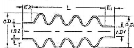
Type E Tapered, Cuff Both Ends
