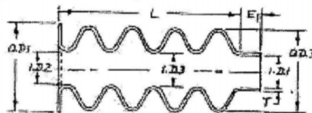
Type D Tapered, One Flange & Cuff End
