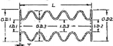
Type E Tapered, Cuff Both Ends
