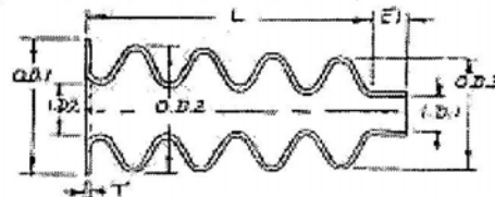
Type F Tapered, One Bead & One Cuff End
