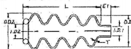
Type F Tapered, One Bead & One Cuff End
